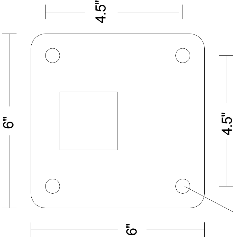
Base Plate Enlarged Top View
